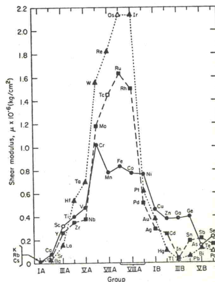
FIG. 3. Shear modulus of the elements of the fourth, fifth, and sixth periods of the Periodic Table. Open points are estimated values.
